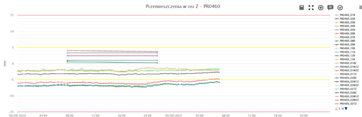
Figure 6-4 Settlement of building PR0460
