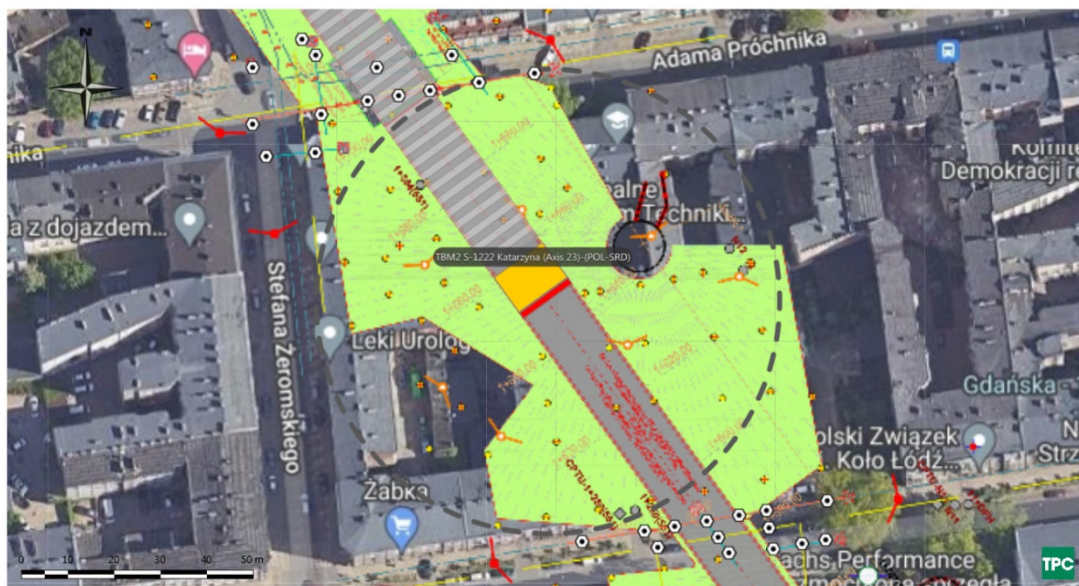
Figure 1-2 Plan view of TBM Position on 04/09/2024
