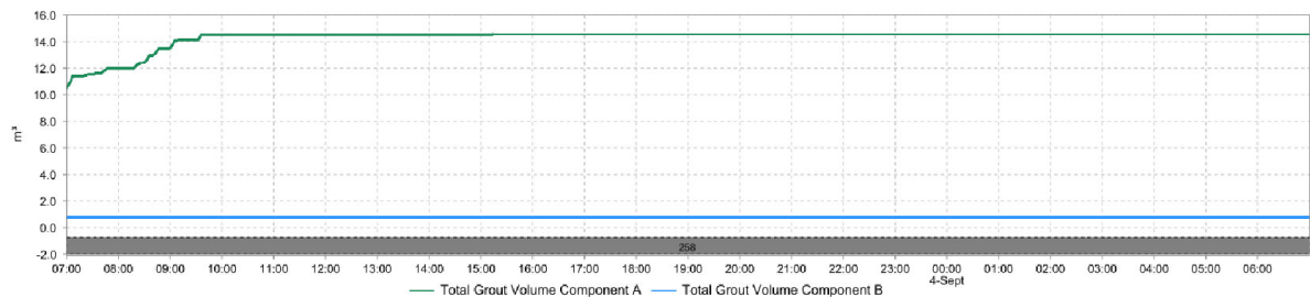
Figure 4-1 Grout volumes
